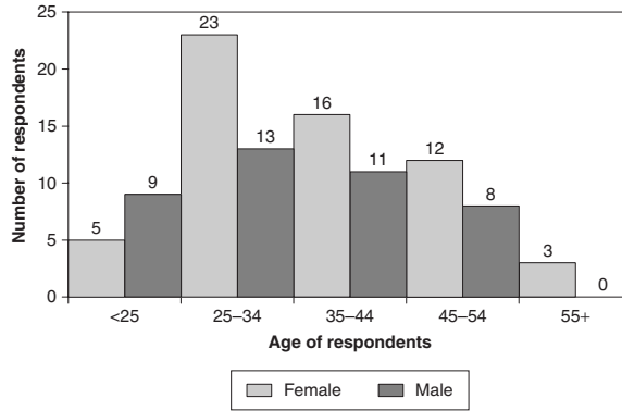
FIGURE 16.2c Two-dimensional histogram with two variables
