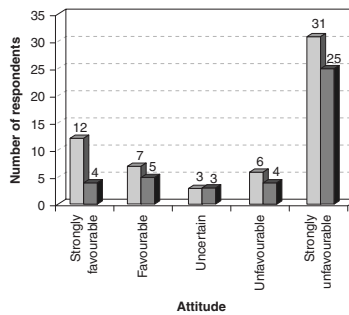
d: two variables (3D)
