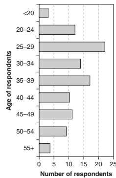
c: one variable (vertical box)
